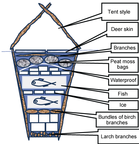
Figure 2 Structure of an ice well (Ivelovsky sand area, Nadym).[11]
